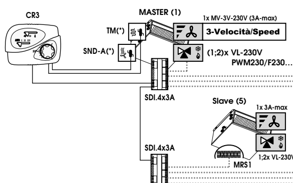
Fig.6...10: MASTER-SLAVE con logica Open-Space - Fig.6...10: MASTER-SLAVE with Open-Space logic
