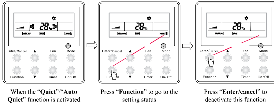
Fig.25 How to Deactivate the “Quiet”/“Auto Quiet” Function
