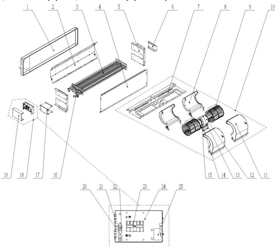
FP-51WA(H)/G Part Lists:
