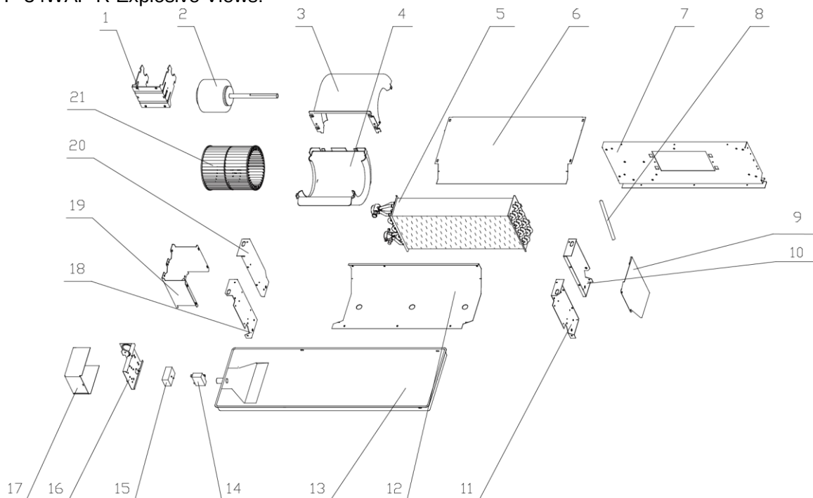
FP-34WAF-R Explosive Views:
